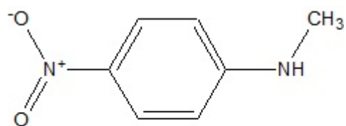
N-Methyl-4-nitroaniline
